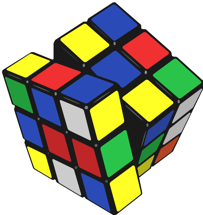
Rubik's Cube
